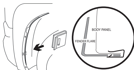
Push U-Clip
